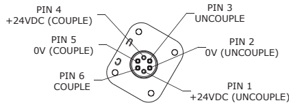
VIEW B-B SCALE 2:1
